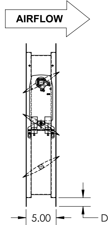
SIDE VIEW (BLADES OPEN)
