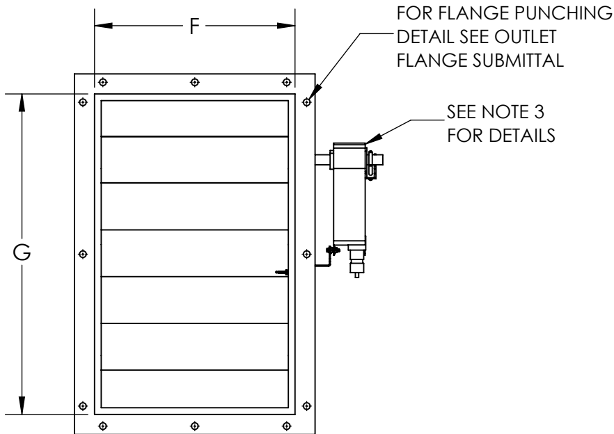
BACK VIEW (BLADES OPEN)
